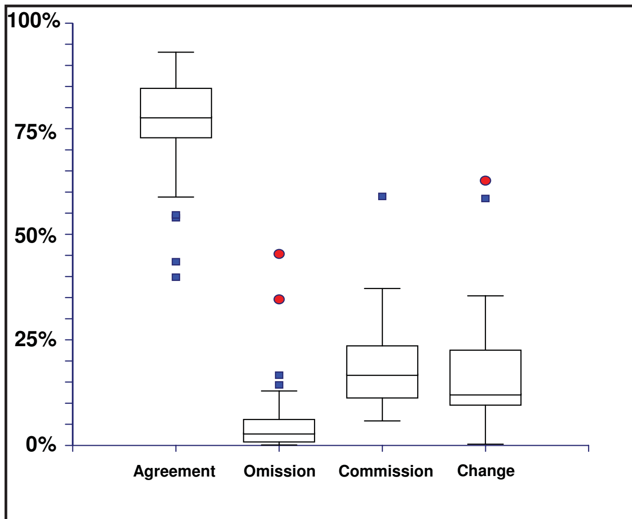
Figure 4. Range of variability in three fire mapping agreement categories and total change in area, shown by box plots, with mild ( 1.5 \times IQR) outliers indicated by squares and severe ( 3.0 \times IQR) outliers indicated by circles. IQR = interquartile range.
