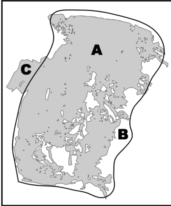
Figure 3 Percent agreement (A) calculated based on overlap of BLM-mapped polygons and the post-processing polygons from remotely sensed data, with error of commission (B) where it did not burn and error of omission (C) where it did burn but was not mapped as such.
