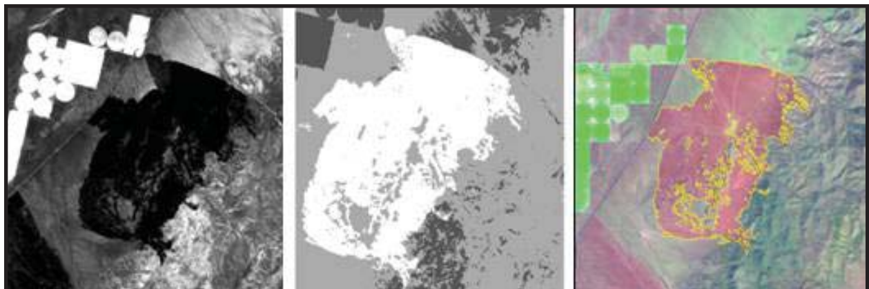
Figure 2. Classification of fires using (from l - r) NBR, unsupervised classification, and a raster to feature transformation.
