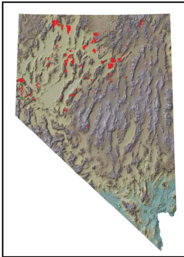
Figure 1. Locations of 53 fires analyzed in Nevada.
